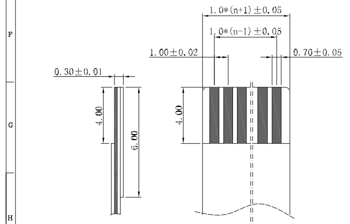
RECOMMENDED FFC/FPC CABLE DIMENSION
