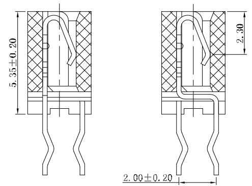
SECTION A-A SECTION B-B
